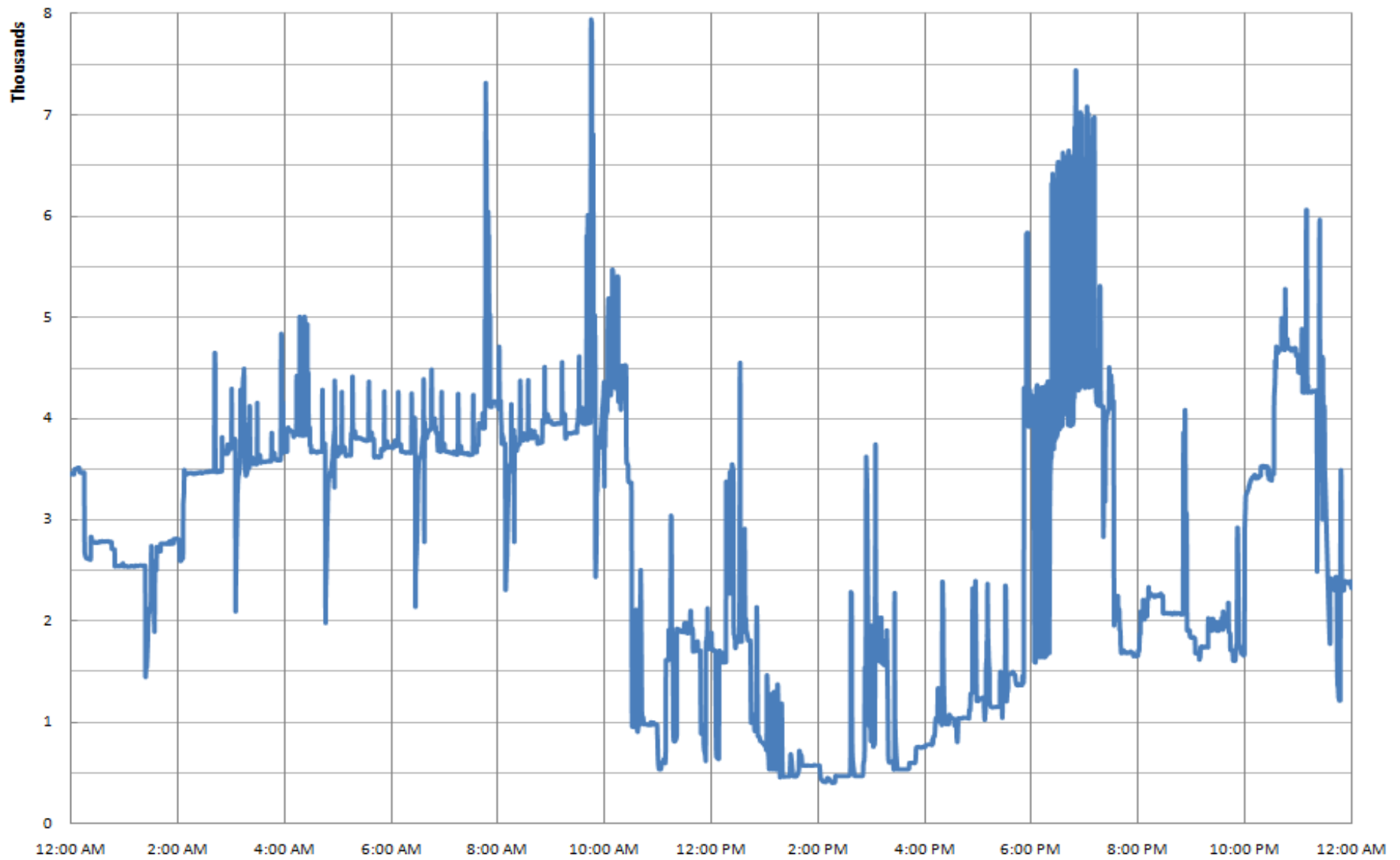
Electric Use, Sat Jan 15, 2011, Watts
